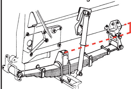
BUMP STOP CLEARANCE
