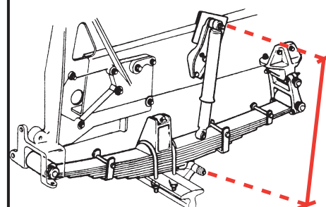
EXTENSION HEIGHT OF SUSPENSION
