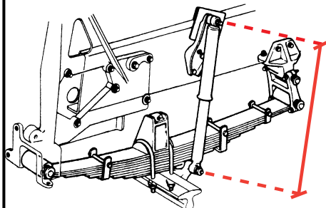
STATIC HEIGHT
